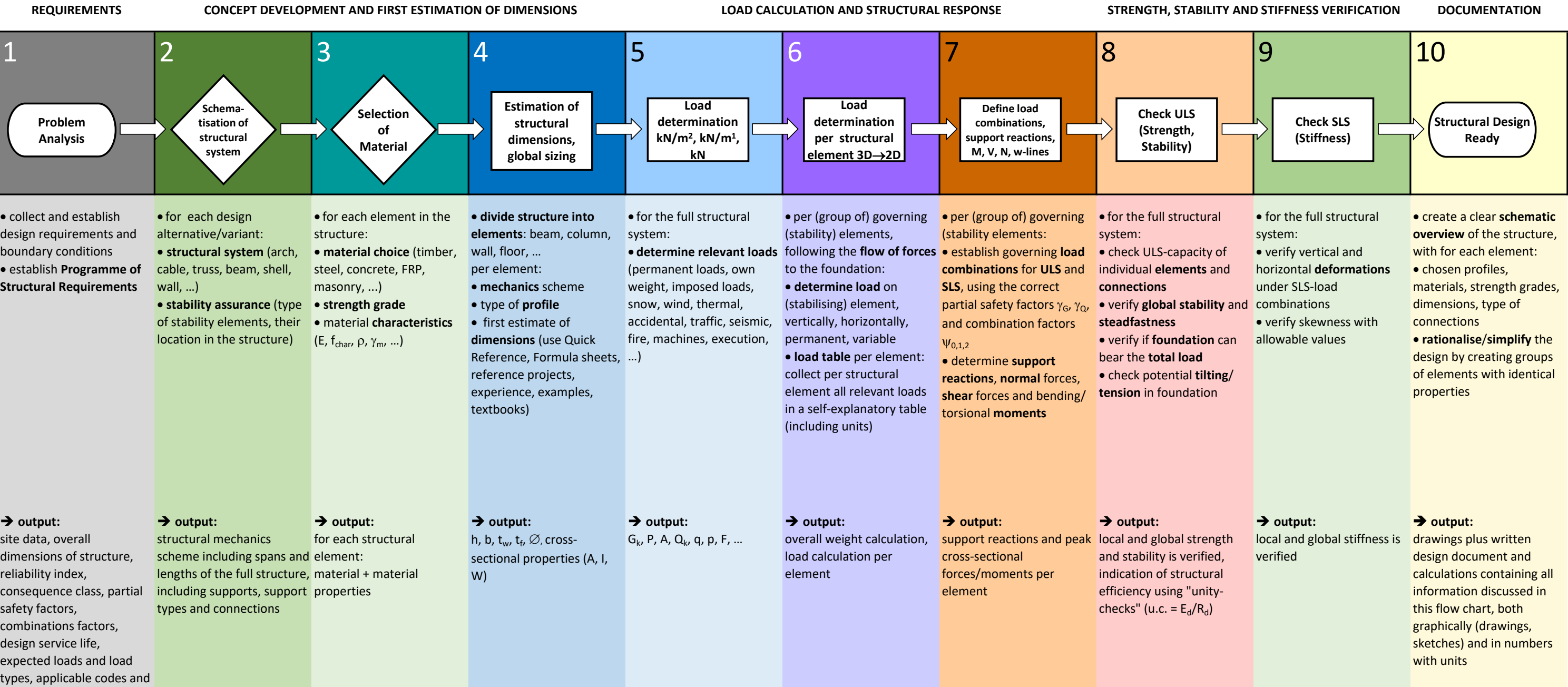
FLOWCHART STRUCTURAL DESIGN (translation from scheme developed by Lisette Klompenhouwer, BSc (2015))
